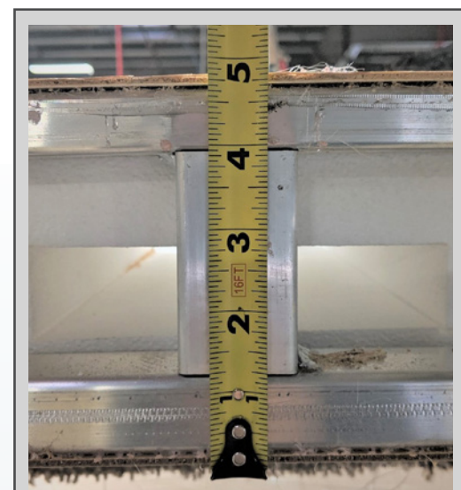
VACUUM BONDED ROOF Solid 5" Crowned Vacuum Bonded Roof with Extremely High Load Rating Capacity on All Models
